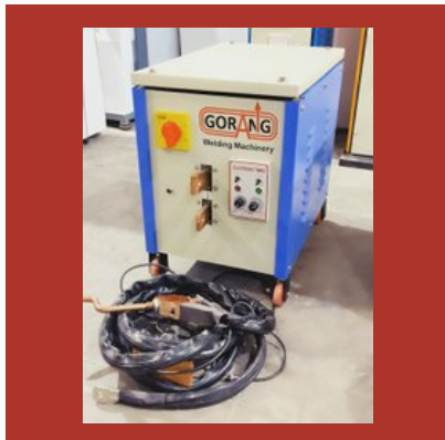
Hand Spot Welding Machine
